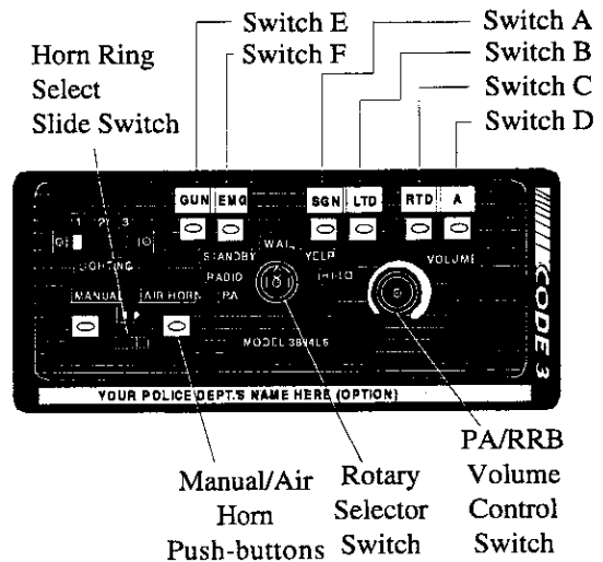
Figure 1 - Control Panel
